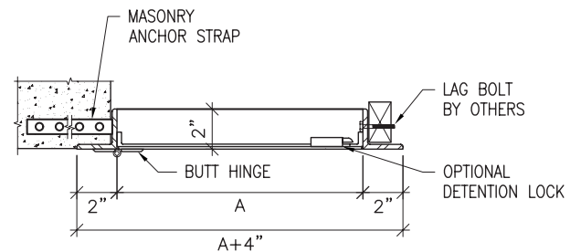
Section Detail
