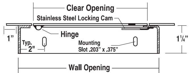
Section Detail
