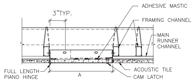
Section Detail
