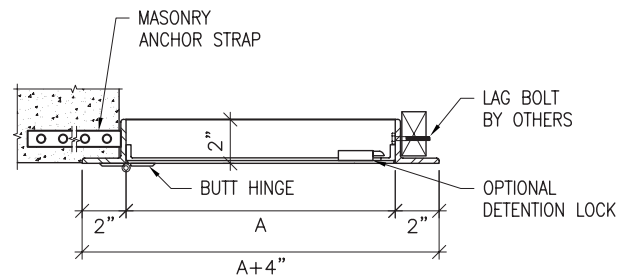
Section Detail
